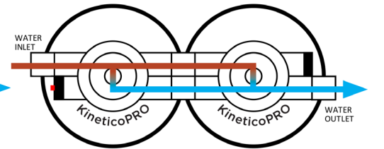
Series Parallel Manifold Configuration
