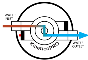
Split Manifold Configuration
