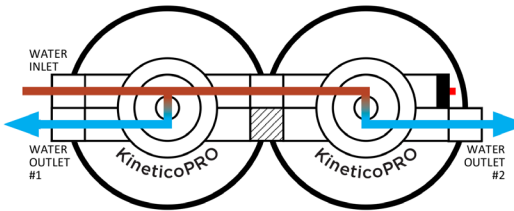
Series Parallel Manifold Configuration
