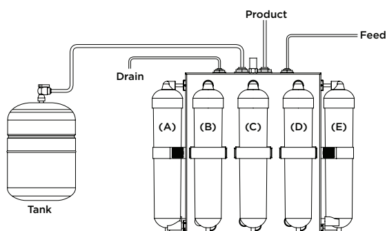
Figure 1: Component Identification
