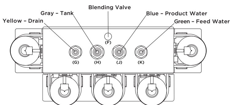
Figure 2: Bulkhead Identification
