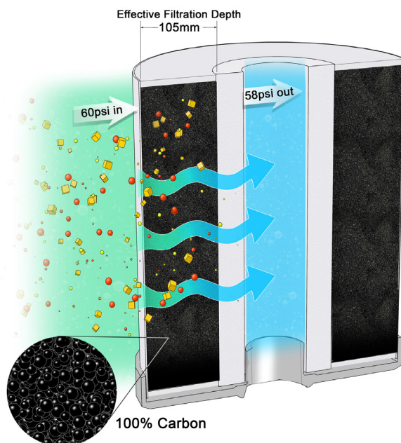
KINETICOPRO'S HOLLOW CARBON FILTERS (Low Pressure Drop)
