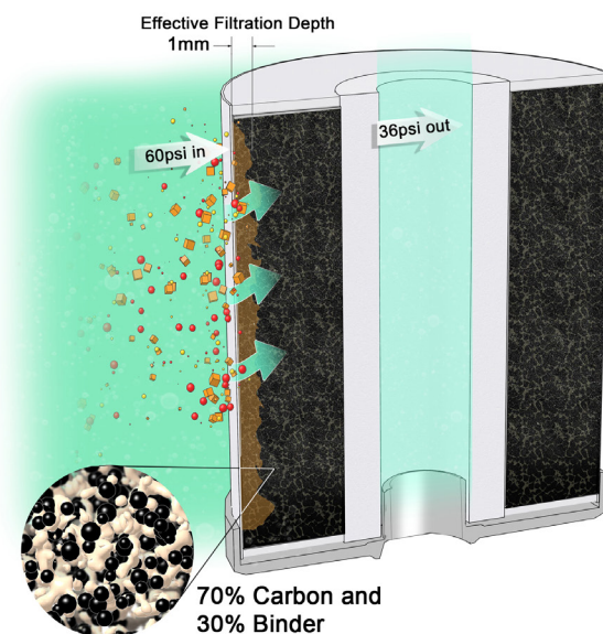
STANDARD CARBON BLOCK (High Pressure Drop)
